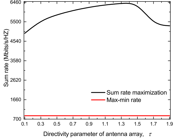
Fig. 2. Effect of \tau on sum rate.
